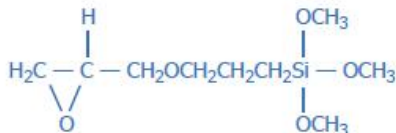
Gamma-Glycidoxypropyl trimethoxysilane
